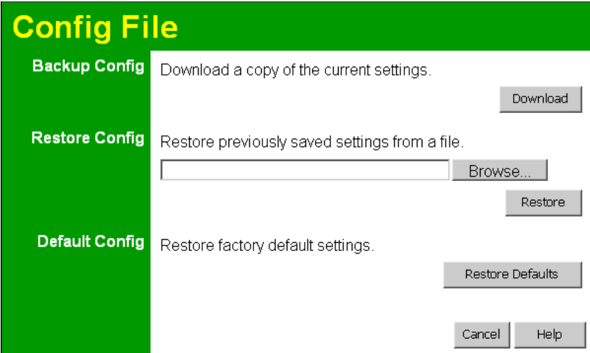
Figure 41: Config Screen
