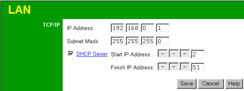
Figure 6: LAN Screen
