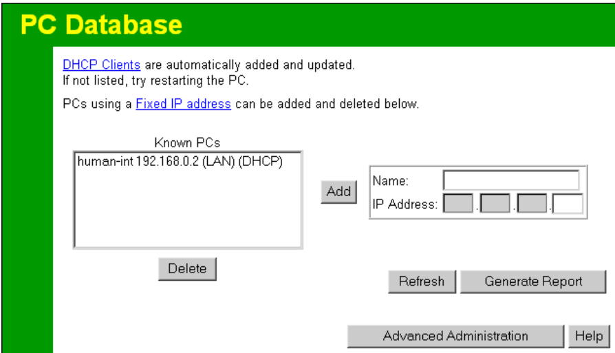
Figure 45: PC Database
