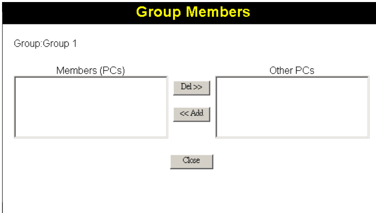
Figure 31: Group Members
