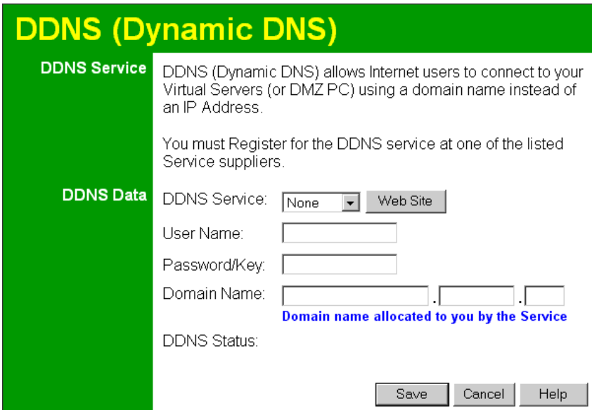
Figure 34: DDNS Screen
