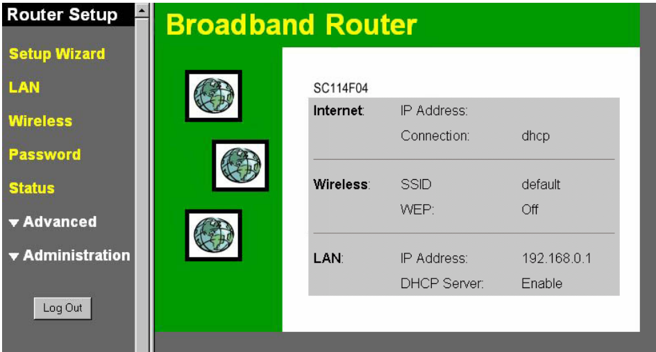
Figure 5: Home Screen
