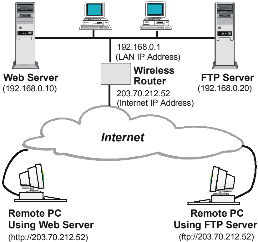
Figure 38: Virtual Servers
