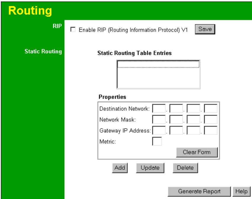
Figure 48: Routing Screen
