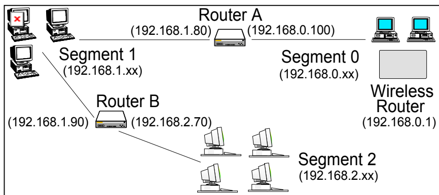
Figure 49: Routing Example
