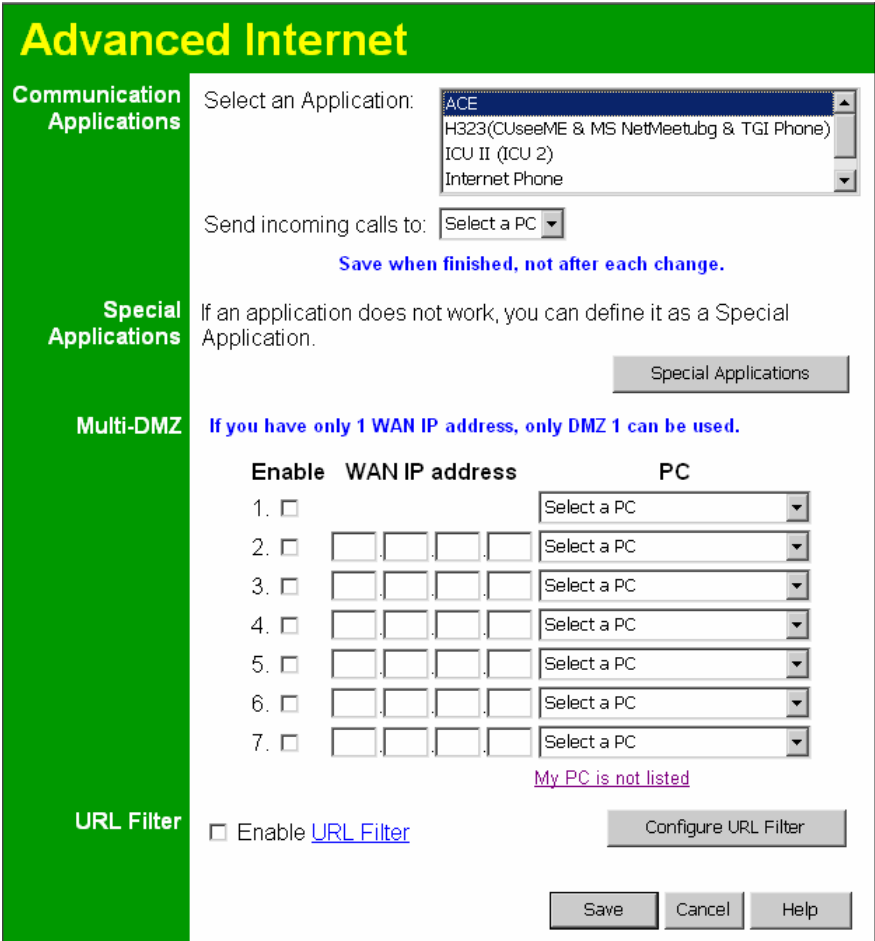
Figure 35: Internet Screen
