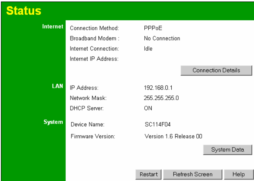
Figure 23: Status Screen
